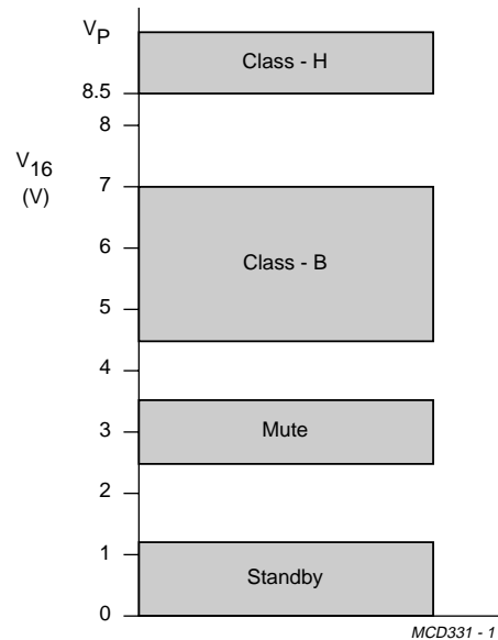
Fig.4 Switching levels of mode select switch.
